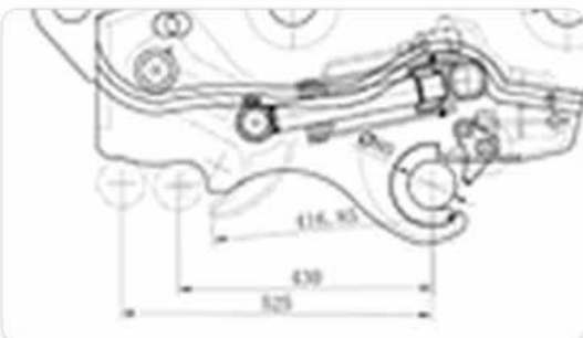
longer cylinder stroke (100mm for 20 ton machine)
